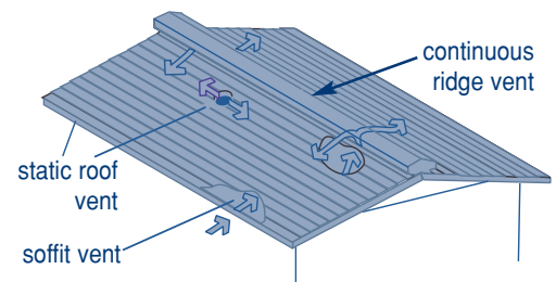
Figure 6: Effective attic ventilation. Intake venting low through the soffit and exhaust venting high through a continuous ridge vent are the most effective way to ventilate an attic.
